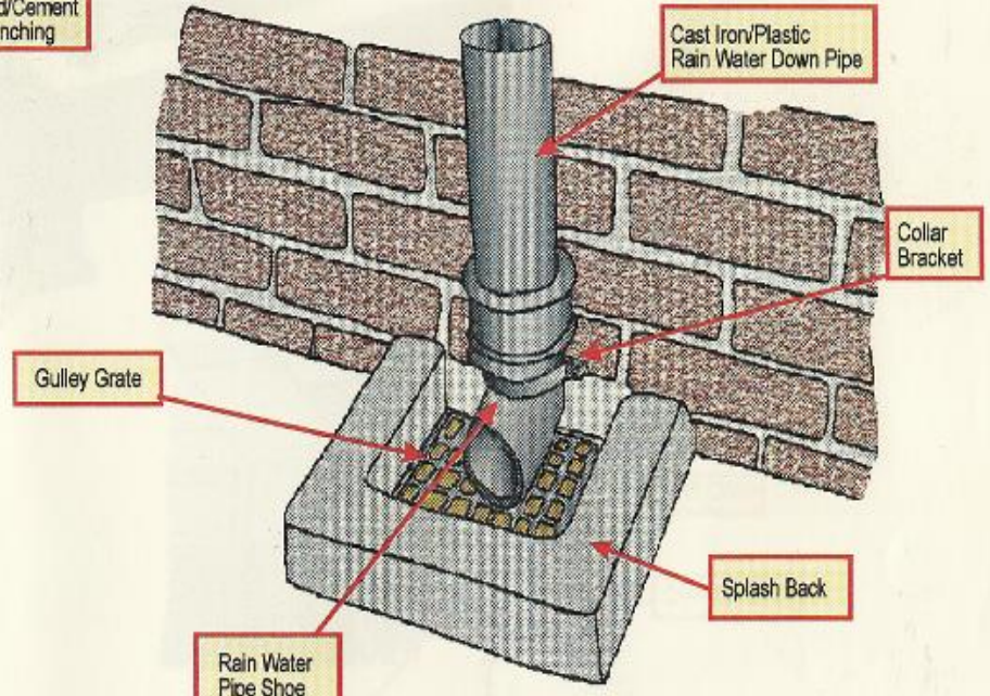
Gully
