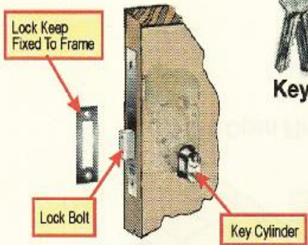
Mortice Cylinder Deadlock
