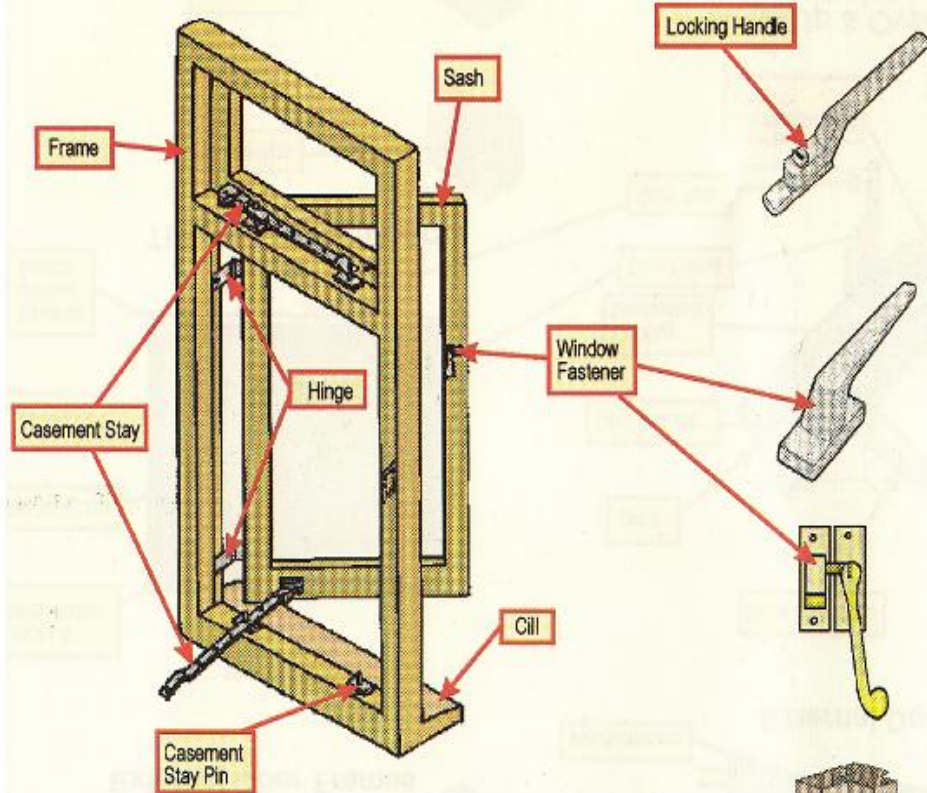
Timber Casement Window
