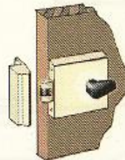
Roller Rim Lock (Single Entrance Flats)
