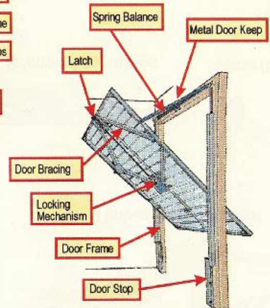
Metal Up & Over (overhead spring balance type)
