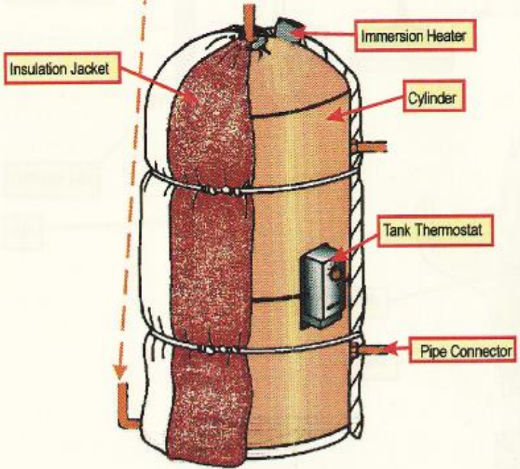
Copper Cylinder
