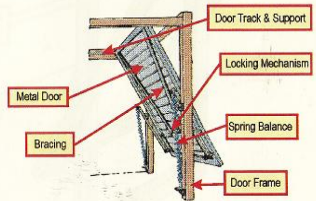
Metal Up & Over (spring balance type)
