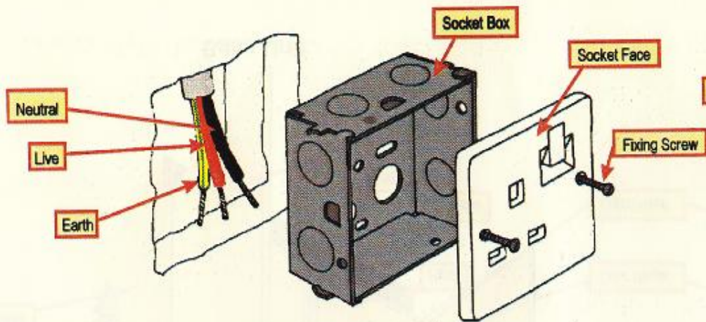
Single Switch Socket
