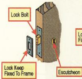
Mortice Deadlock
