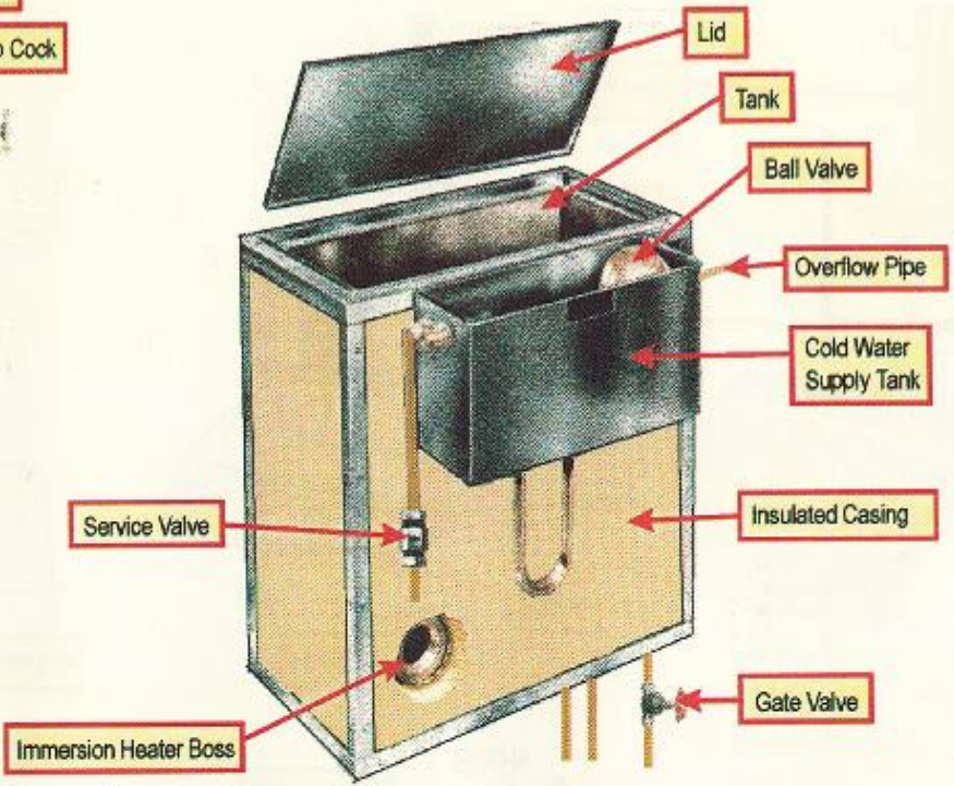
Combination Tank
