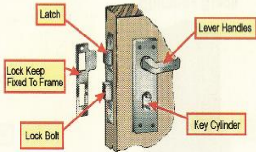
Mortice Cylinder Lock/Latch
