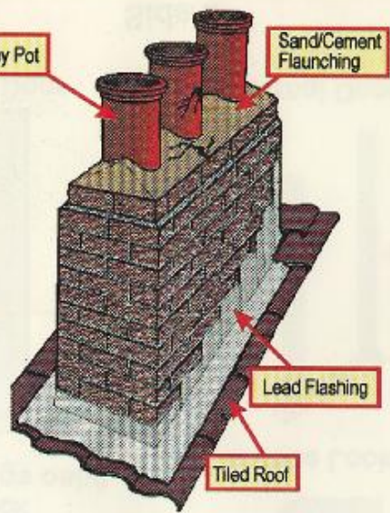
Chimney Stack
