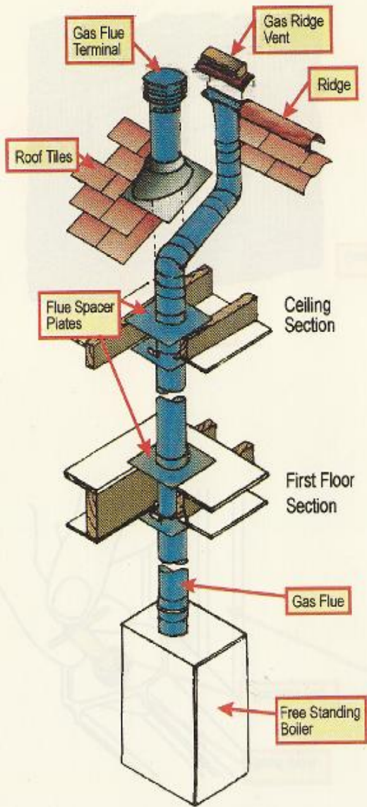
Gas Boiler Flue
