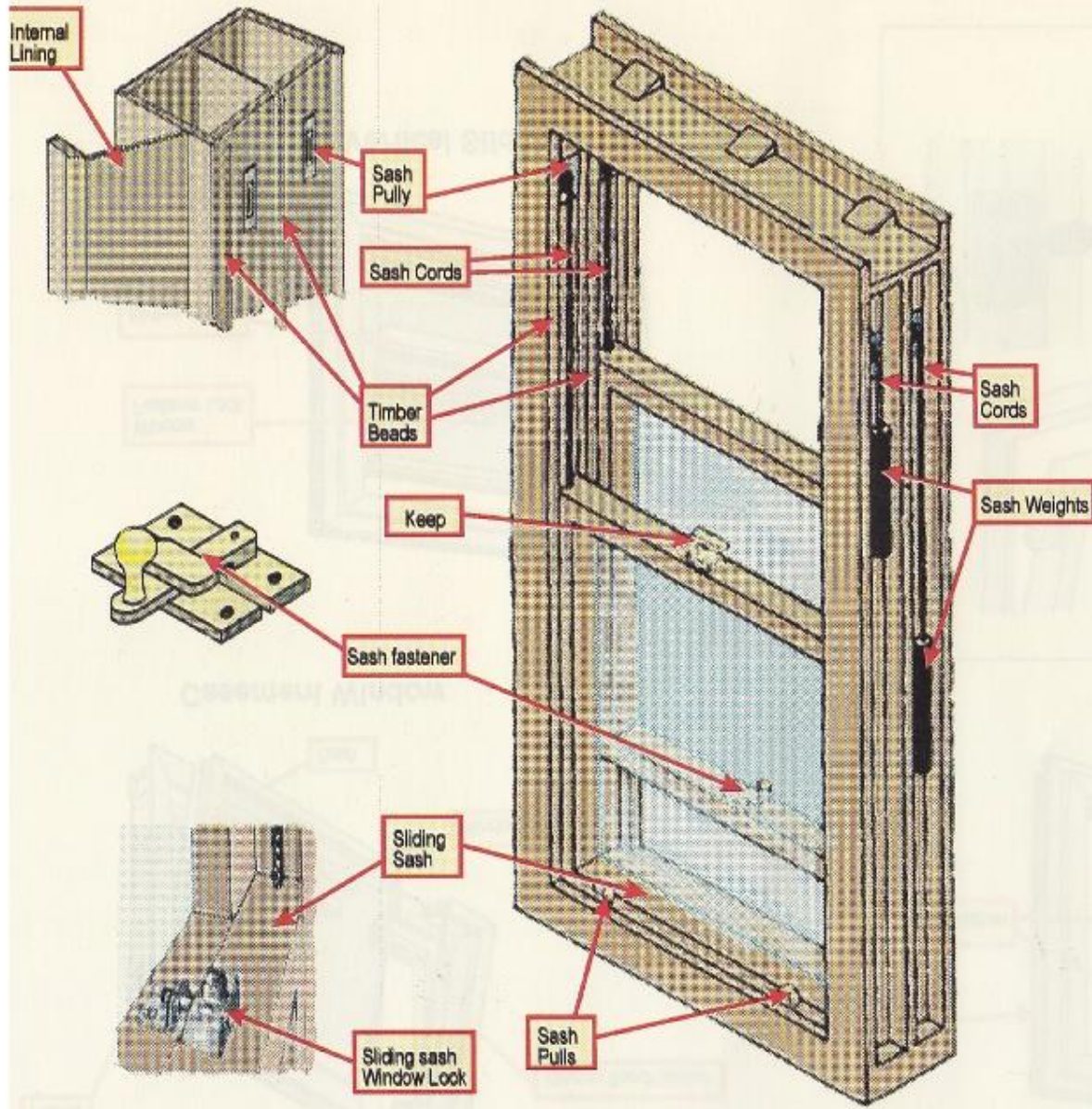
Timber Sliding Sash Window
