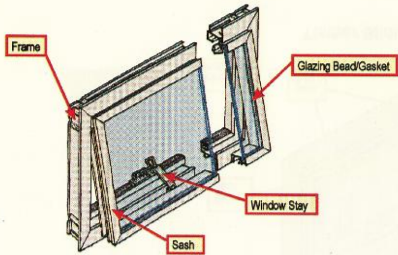
Casement Window
