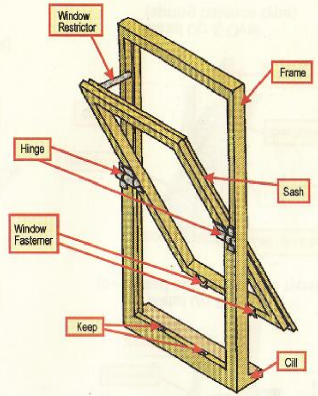
Timber Pivot Window
