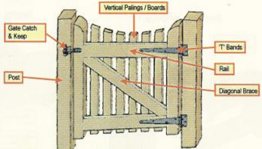
Timber Gate
