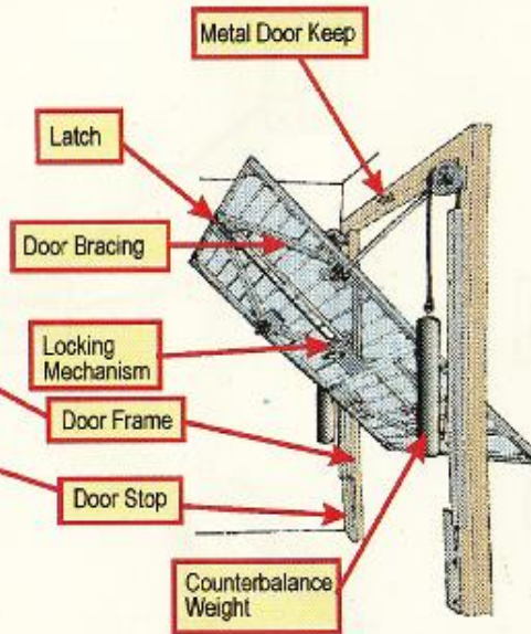
Metal Up & Over (counterbalance type)
