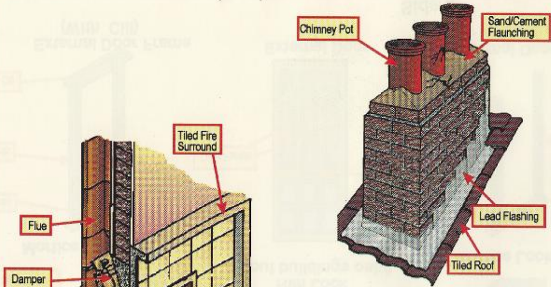
Chimney Stack
