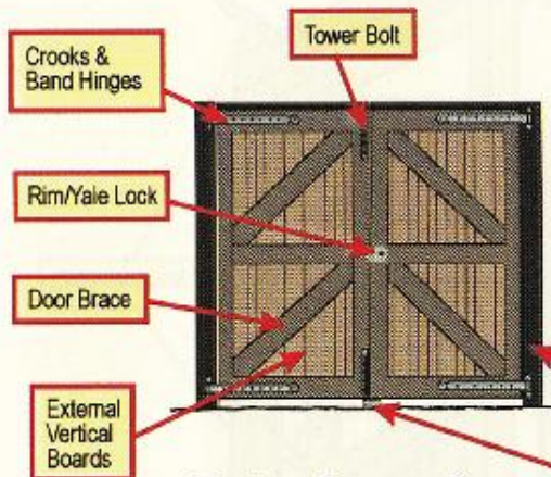
Timber Garage Doors
