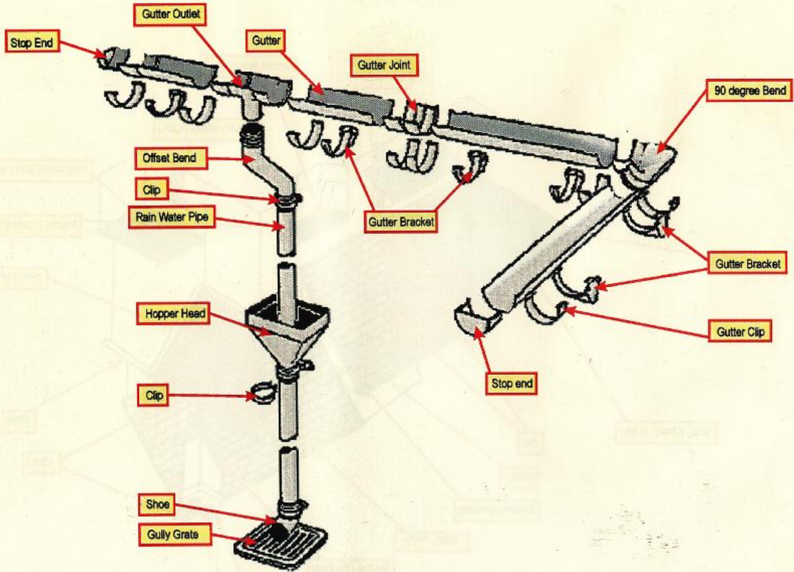
Rain Water System
